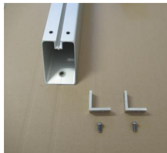
ground bar with hole for ground fixing
