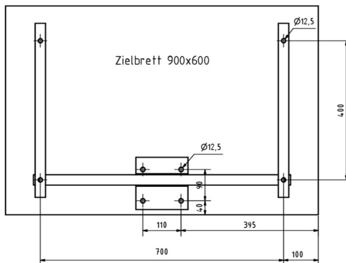
Figure 4: drilling plan basketball board
